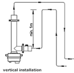
installation above the water level
