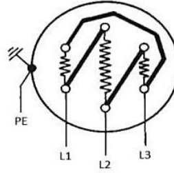
connection for 3x230V (3-phase current)
