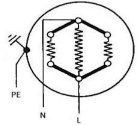
connection to max. 6kW for 1x230V alternating current
